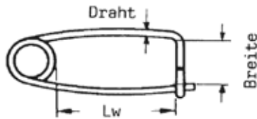
Fokkernadel
